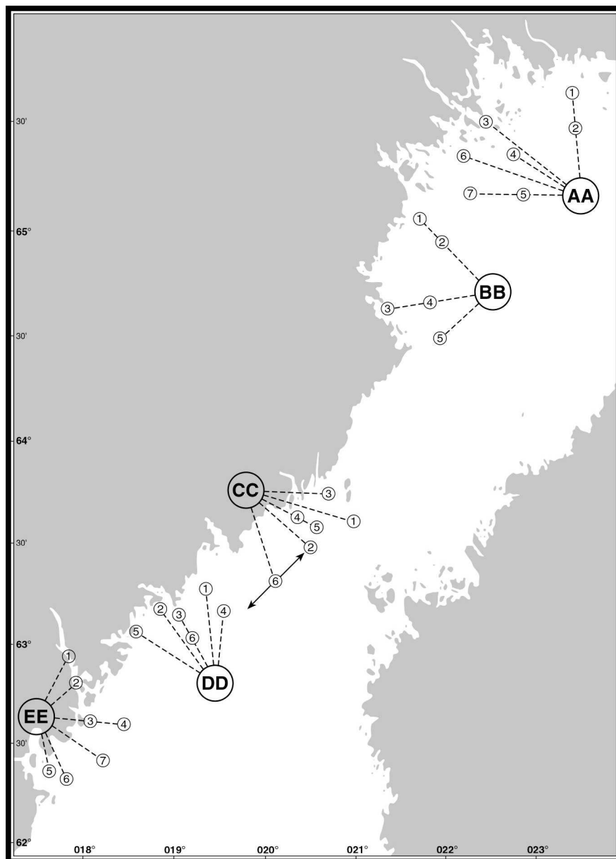
Ice report areas AA to EE
